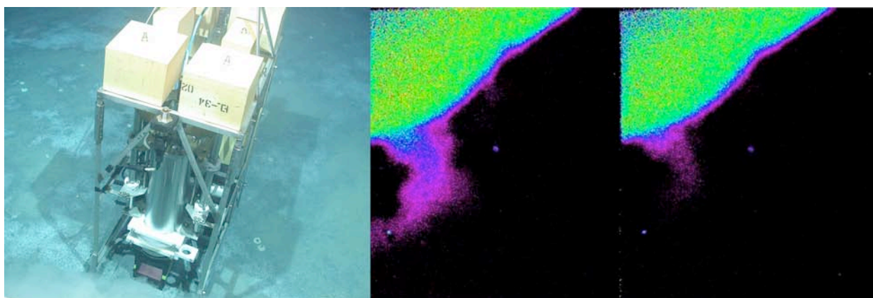
Figure 7.4: Left: Planar optode measuring 2D oxygen distribution in the seafloor. Right: Data from planar optode showing temporal change in 2D oxygen distribution in a deep-sea shrimp burrow. Images courtesy MPI/MARUM.
